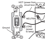
Fig. 1. Typical Single Pole Switch Wiring
