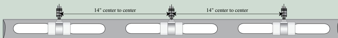
T36" shade five 25 or 40T10F bulbs
