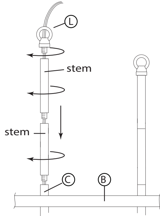
DRAWING 2 - MOUNTING
