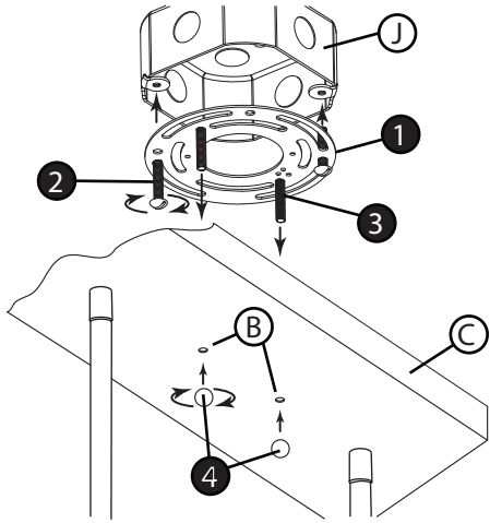
DRAWING 1 - MOUNTING
