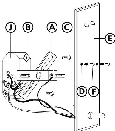
Drawing 2 - Fixture Mounting
