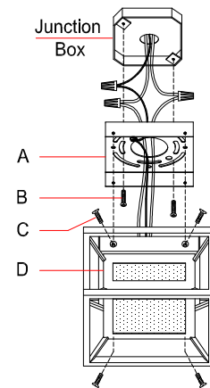
Fig. 2 Ceiling Mount
