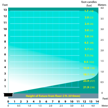
SL-08-AL-FL-7 Half Spread Photometrics (9w)
