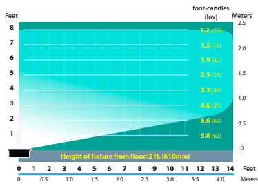
SL-08-AL-FL-5 Half Spread Photometrics (7w)
