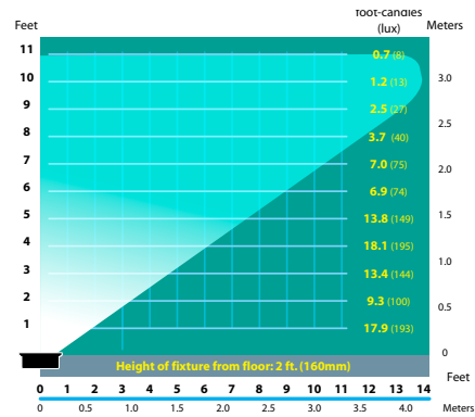
SL-08-T10 Half Spread Photometrics
