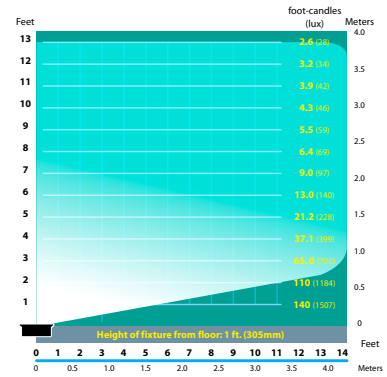
SL-08-FL-9 Half Spread Photometrics (9w)
