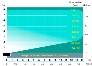
SL-08-AL-FL-5 Half Spread Photometrics (5w)
