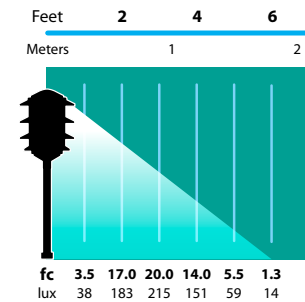
AL-03-4T Half Spread Photometrics 12 ft. (3.7m) diameter
