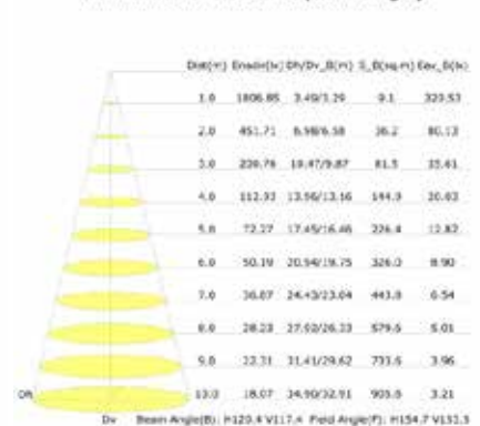
Illuminance at a Distance (Beam Angle)
